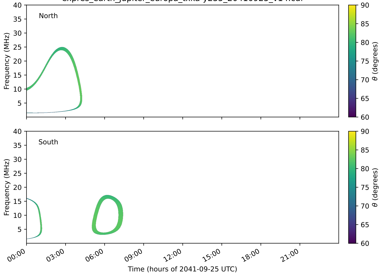
expres_earth_jupiter_europa_txka-y235_20410925_v14.cdf
