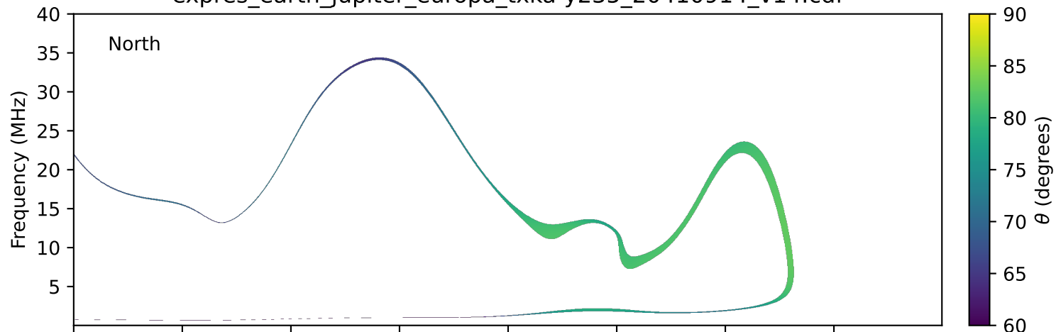
expres_earth_jupiter_europa_txka-y235_20410914_v14.cdf
