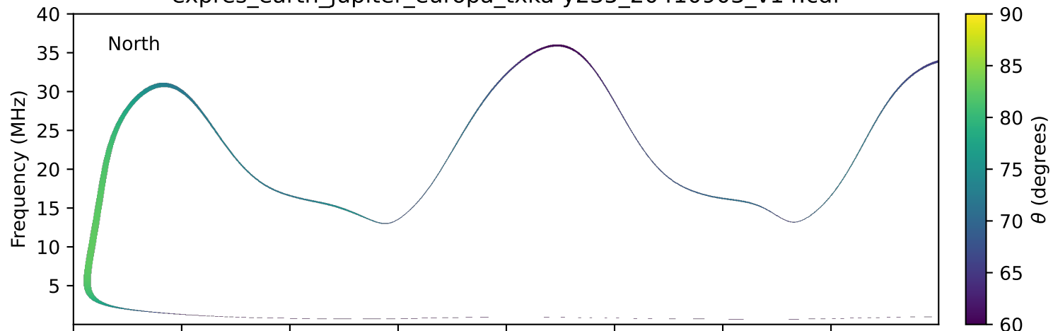
expres_earth_jupiter_europa_txka-y235_20410903_v14.cdf
