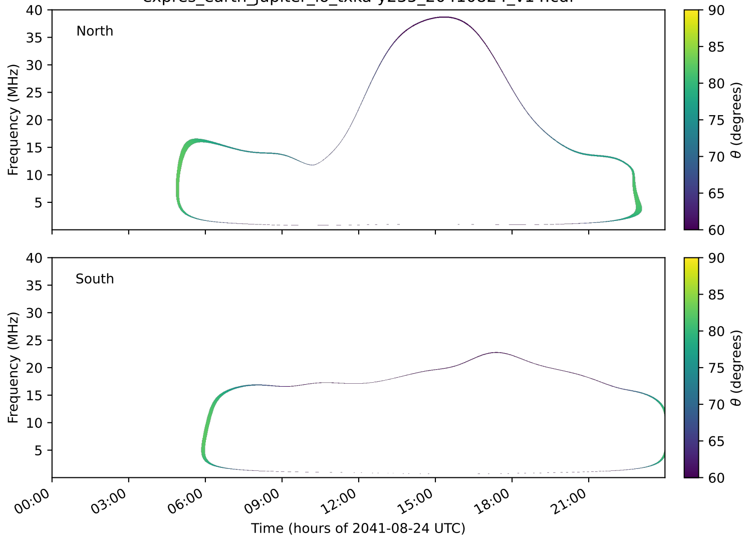
expres_earth_jupiter_io_txka-y235_20410824_v14.cdf
