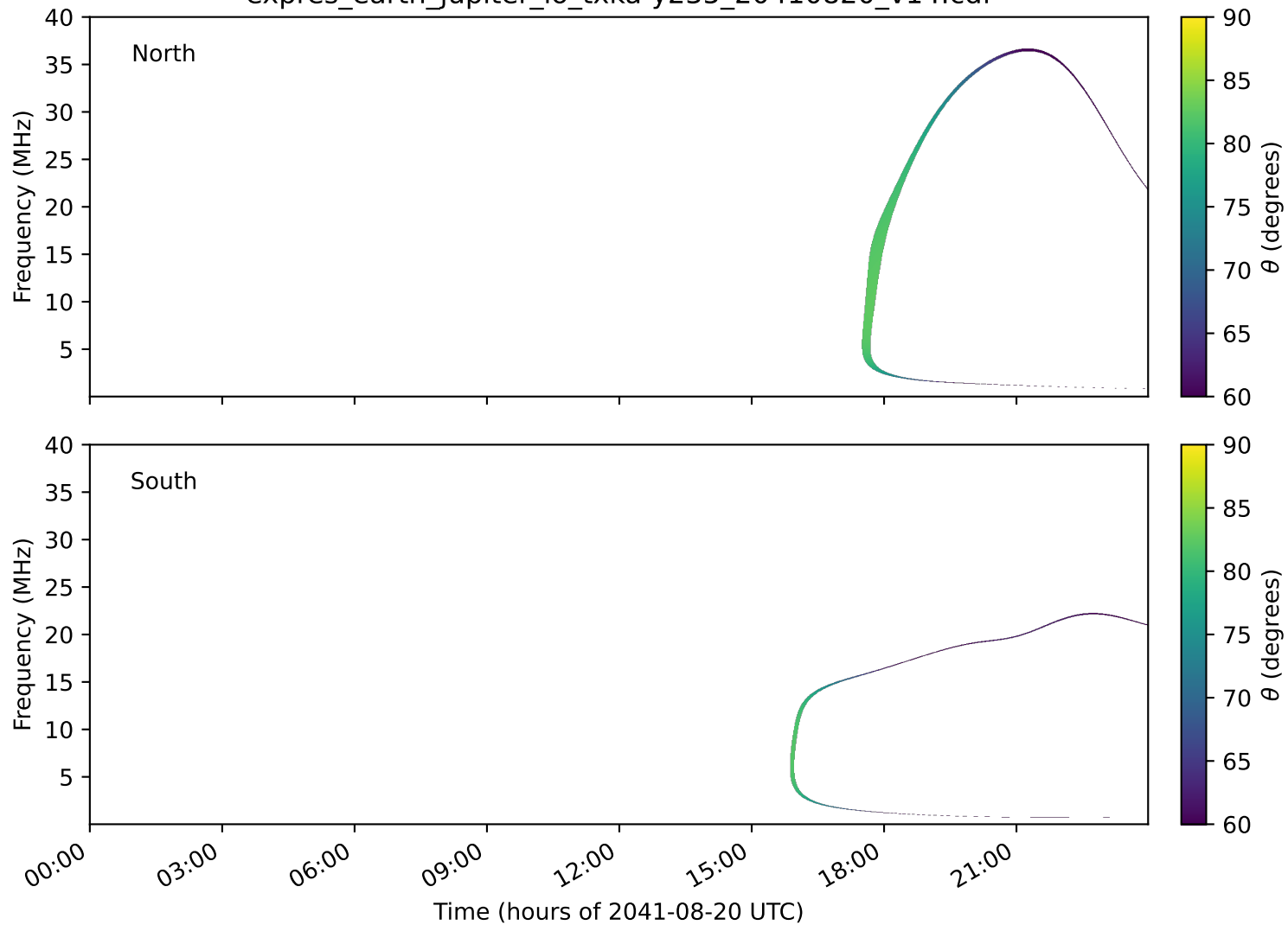
expres_earth_jupiter_io_txka-y235_20410820_v14.cdf
