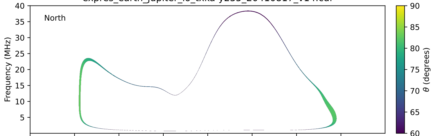
expres_earth_jupiter_io_txka-y235_20410817_v14.cdf
