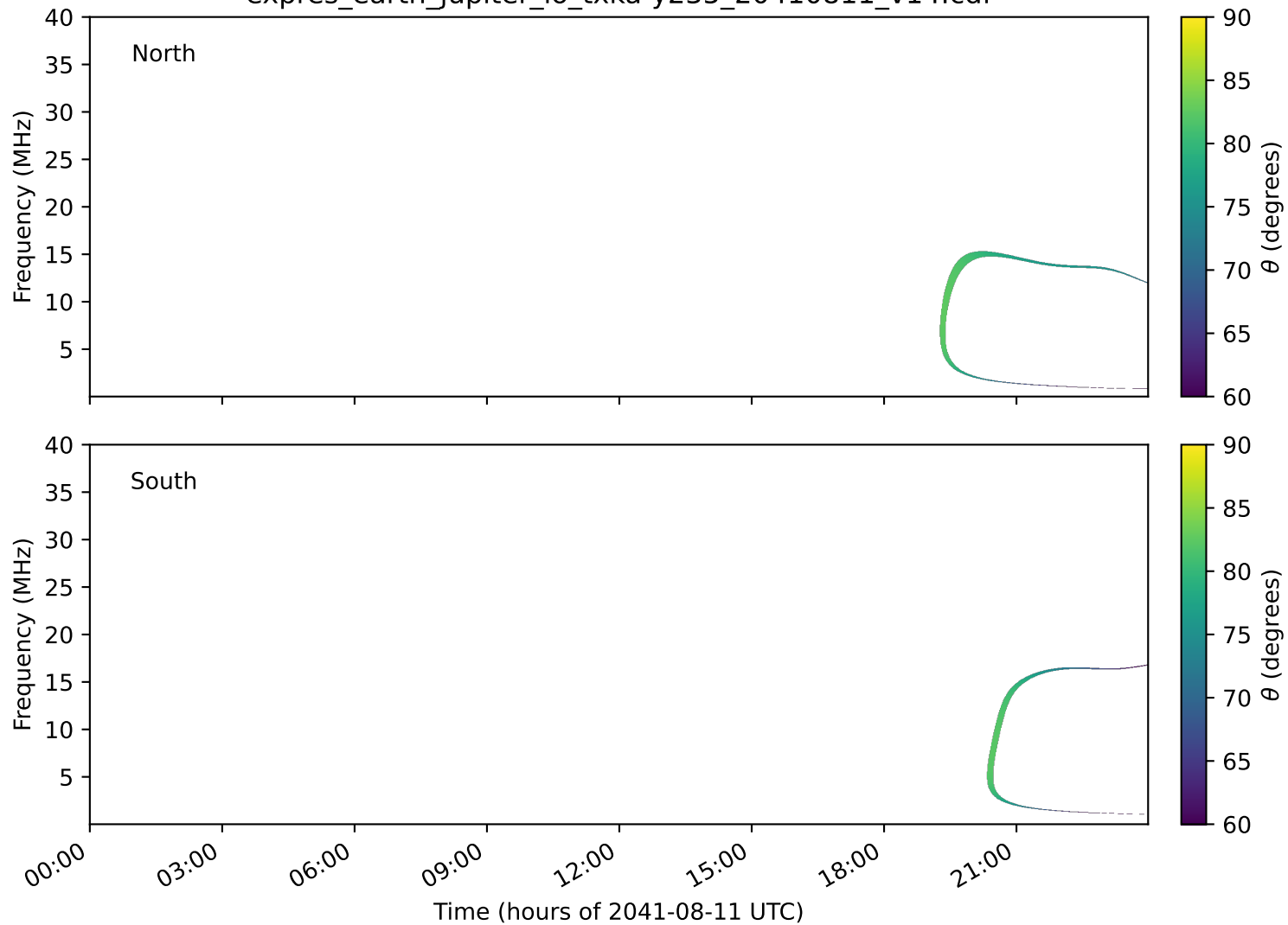
expres_earth_jupiter_io_txka-y235_20410811_v14.cdf
