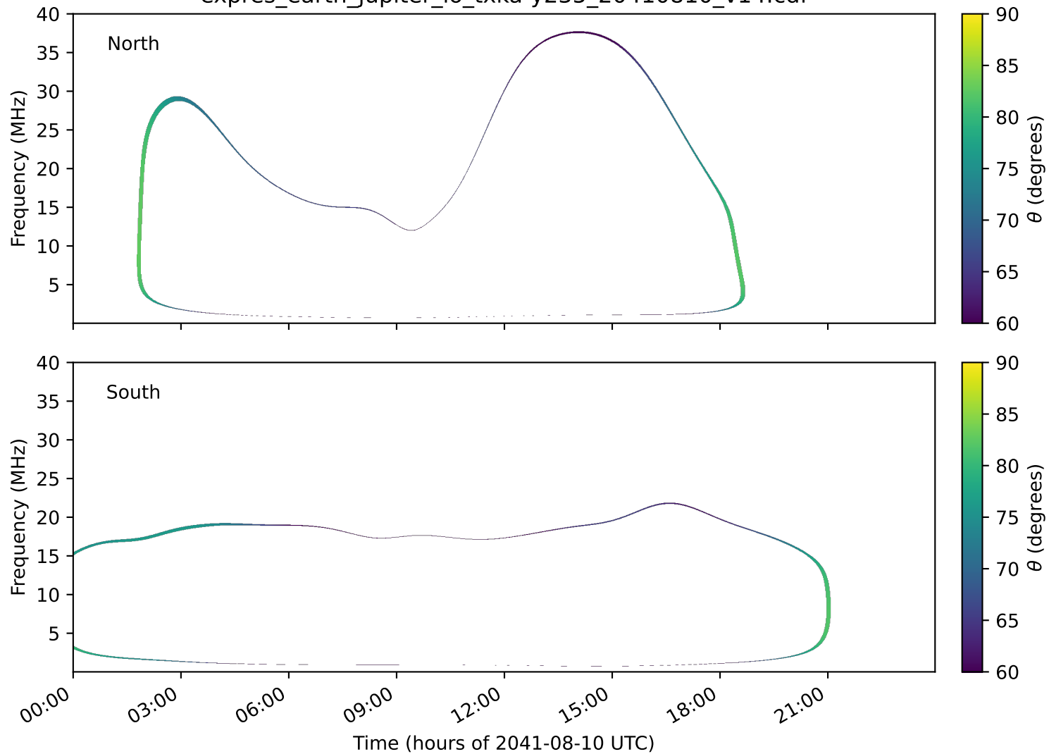
expres_earth_jupiter_io_txka-y235_20410810_v14.cdf
