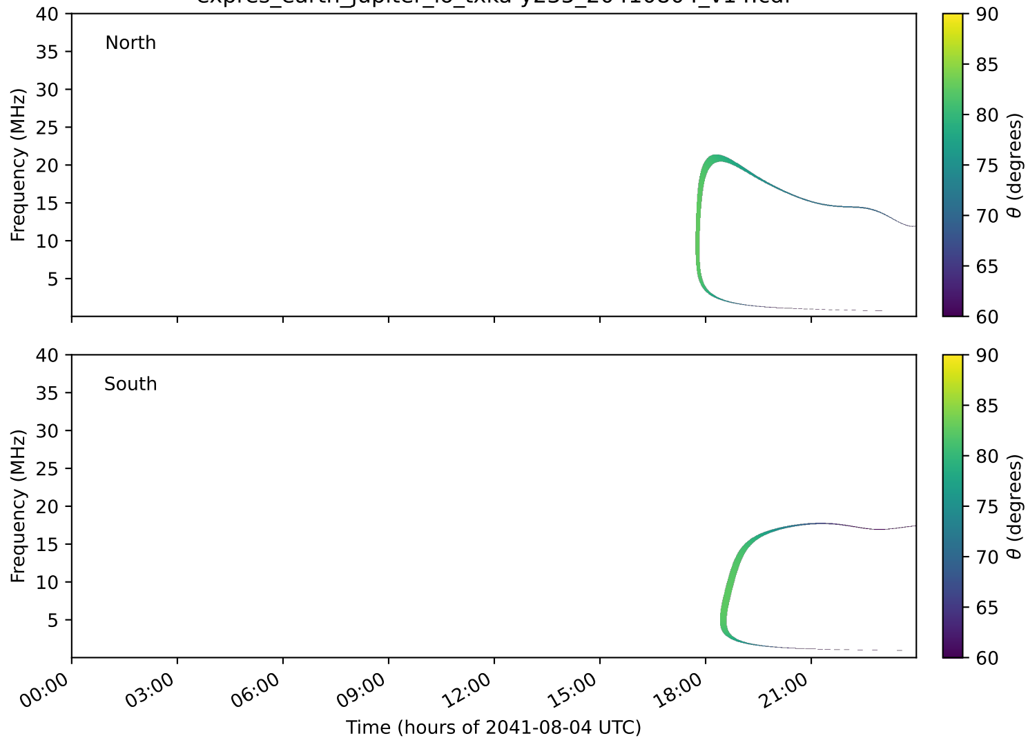
expres_earth_jupiter_io_txka-y235_20410804_v14.cdf
