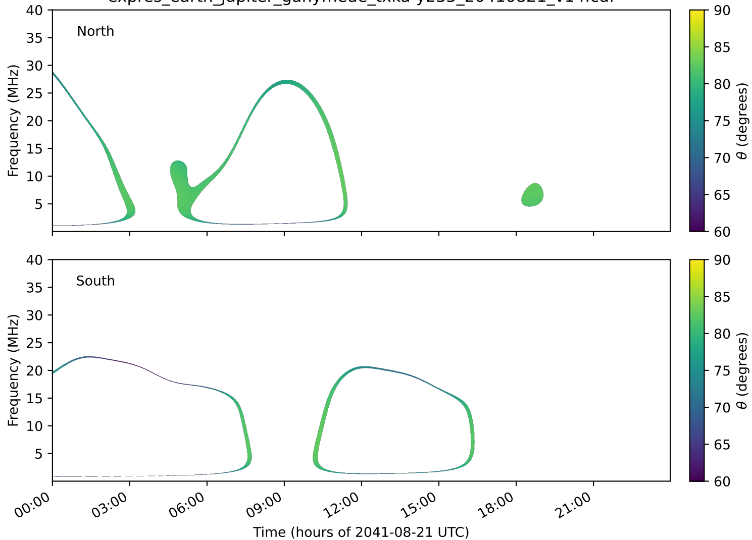
expres_earth_jupiter_ganymede_txka-y235_20410821_v14.cdf
