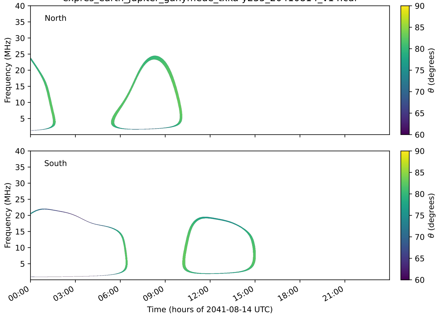
expres_earth_jupiter_ganymede_txka-y235_20410814_v14.cdf
