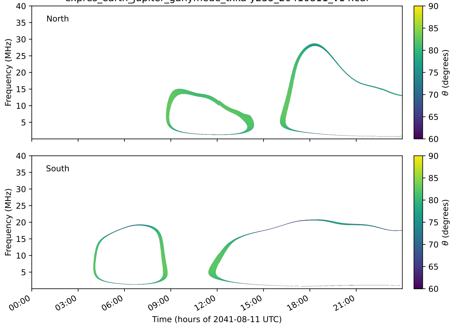
expres_earth_jupiter_ganymede_txka-y235_20410811_v14.cdf
