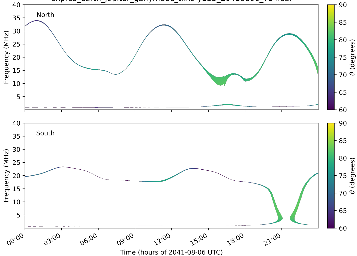
expres_earth_jupiter_ganymede_txka-y235_20410806_v14.cdf
