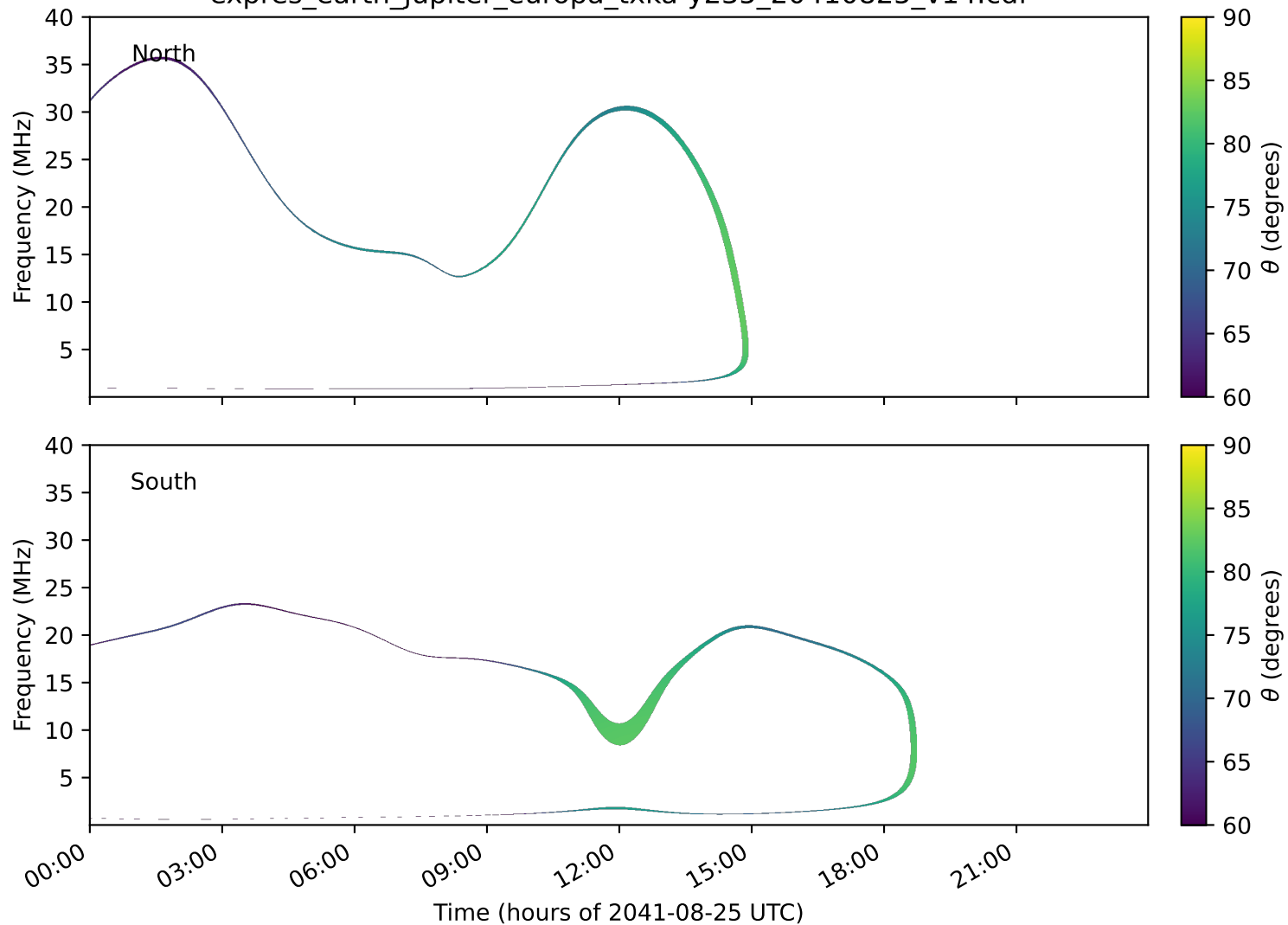
expres_earth_jupiter_europa_txka-y235_20410825_v14.cdf
