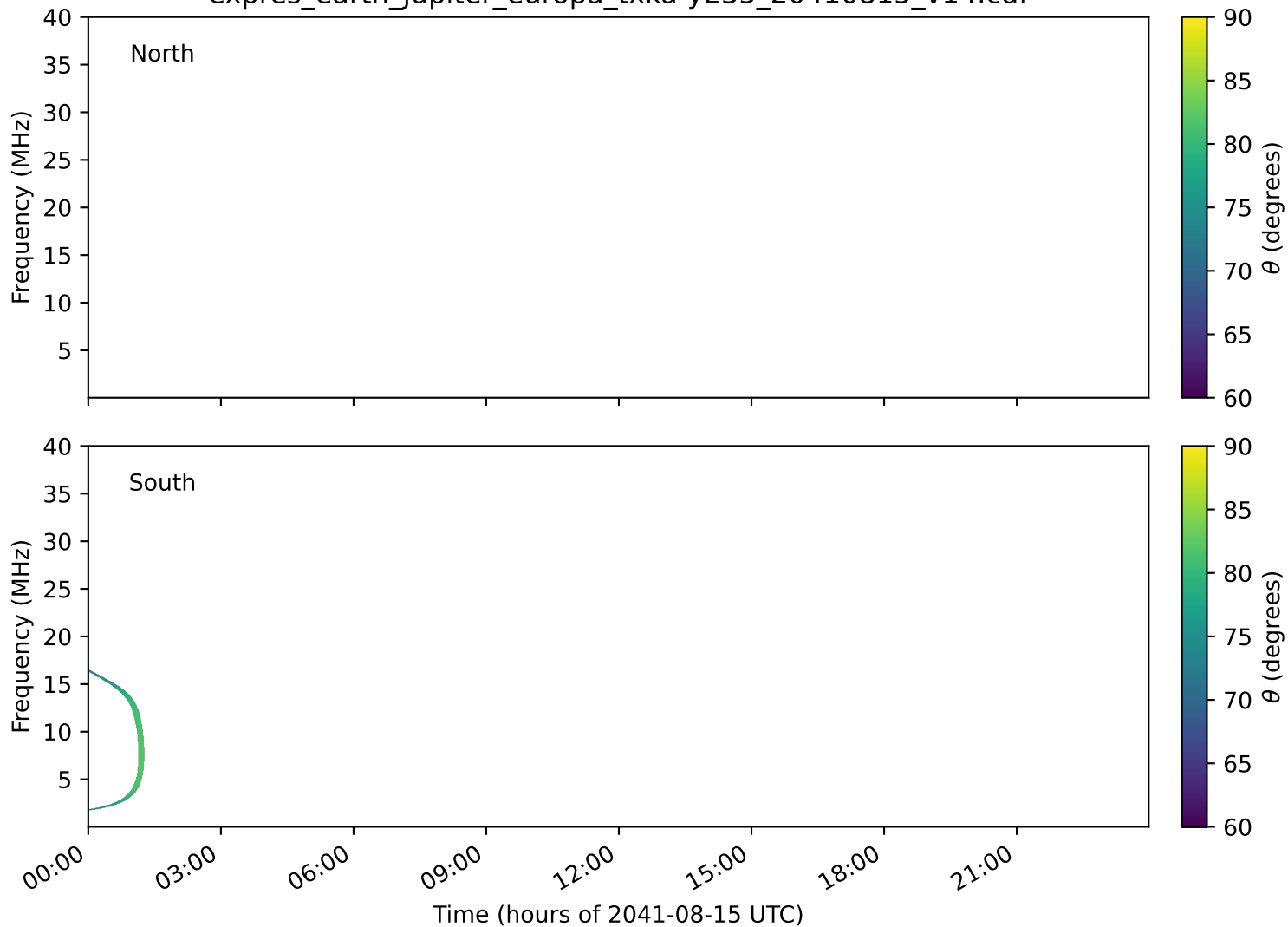
expres_earth_jupiter_europa_txka-y235_20410815_v14.cdf
