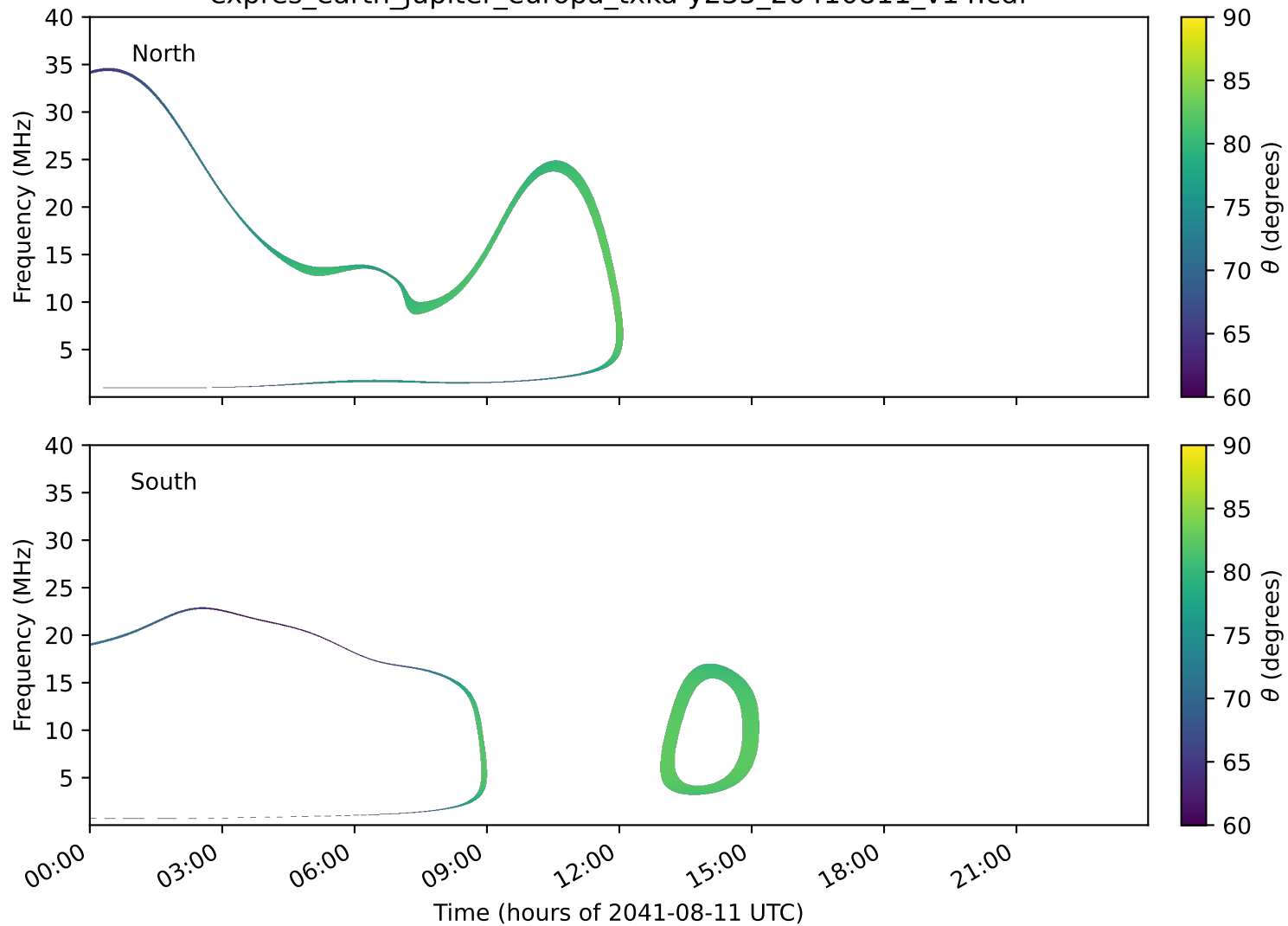
expres_earth_jupiter_europa_txka-y235_20410811_v14.cdf
