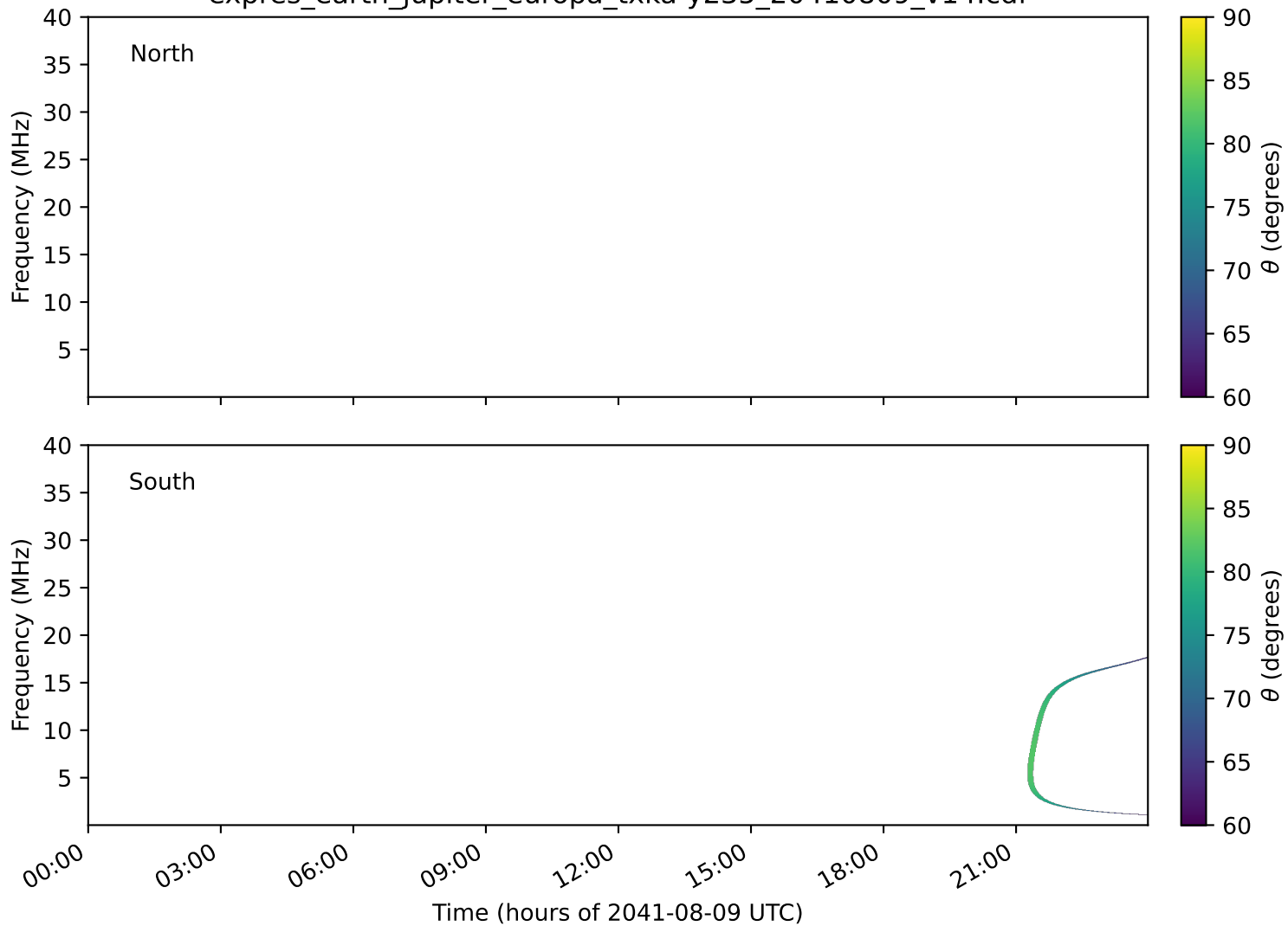
expres_earth_jupiter_europa_txka-y235_20410809_v14.cdf
