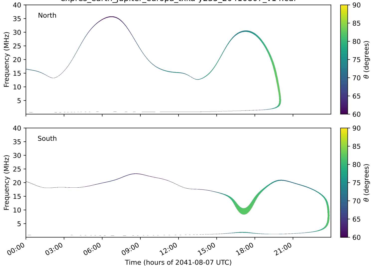
expres_earth_jupiter_europa_txka-y235_20410807_v14.cdf
