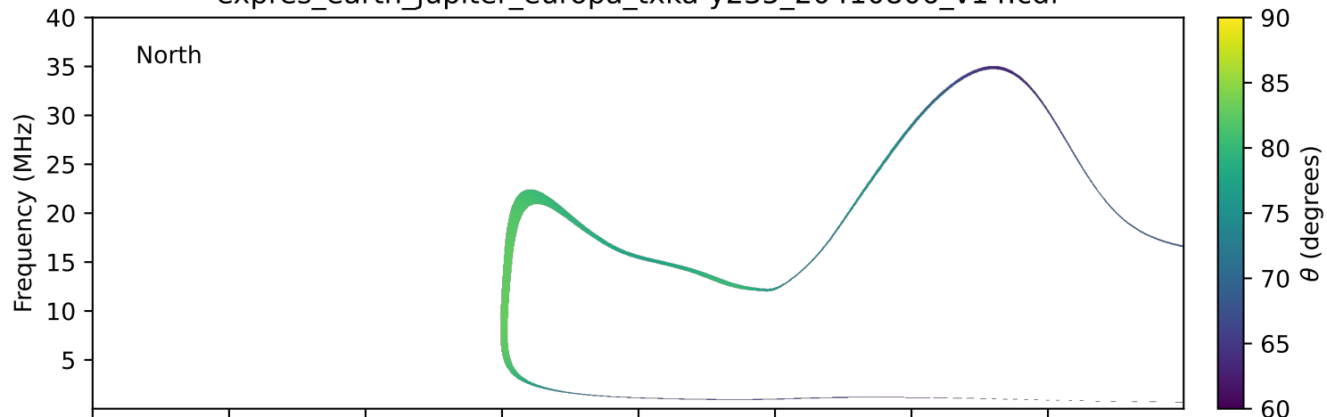
expres_earth_jupiter_europa_txka-y235_20410806_v14.cdf
