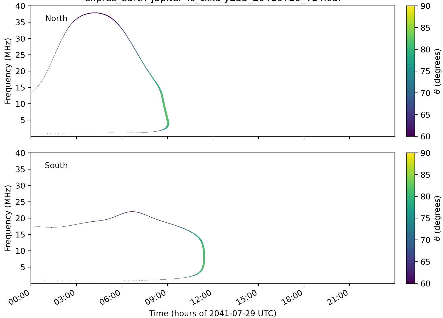
expres_earth_jupiter_io_txka-y235_20410729_v14.cdf
