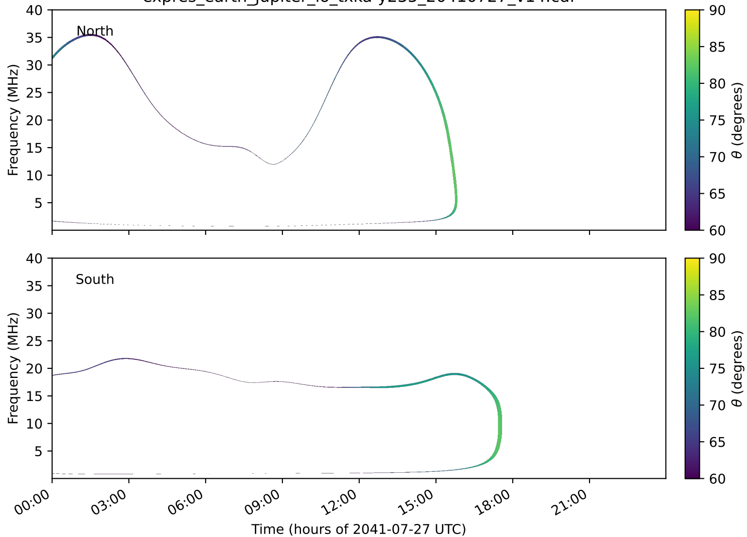
expres_earth_jupiter_io_txka-y235_20410727_v14.cdf
