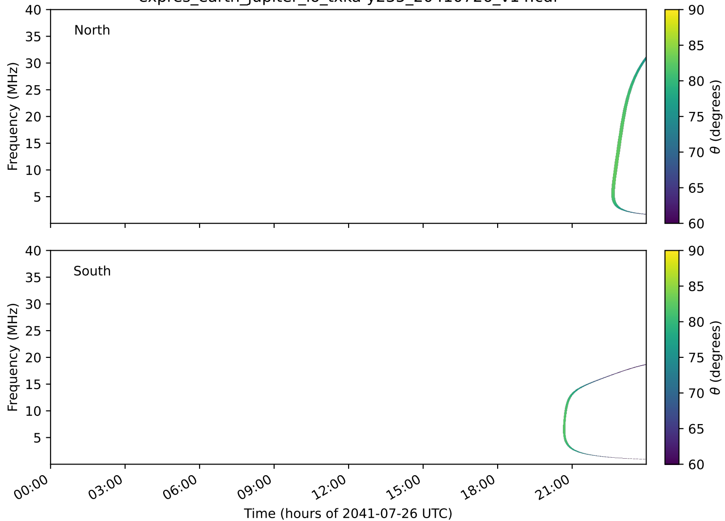
expres_earth_jupiter_io_txka-y235_20410726_v14.cdf
