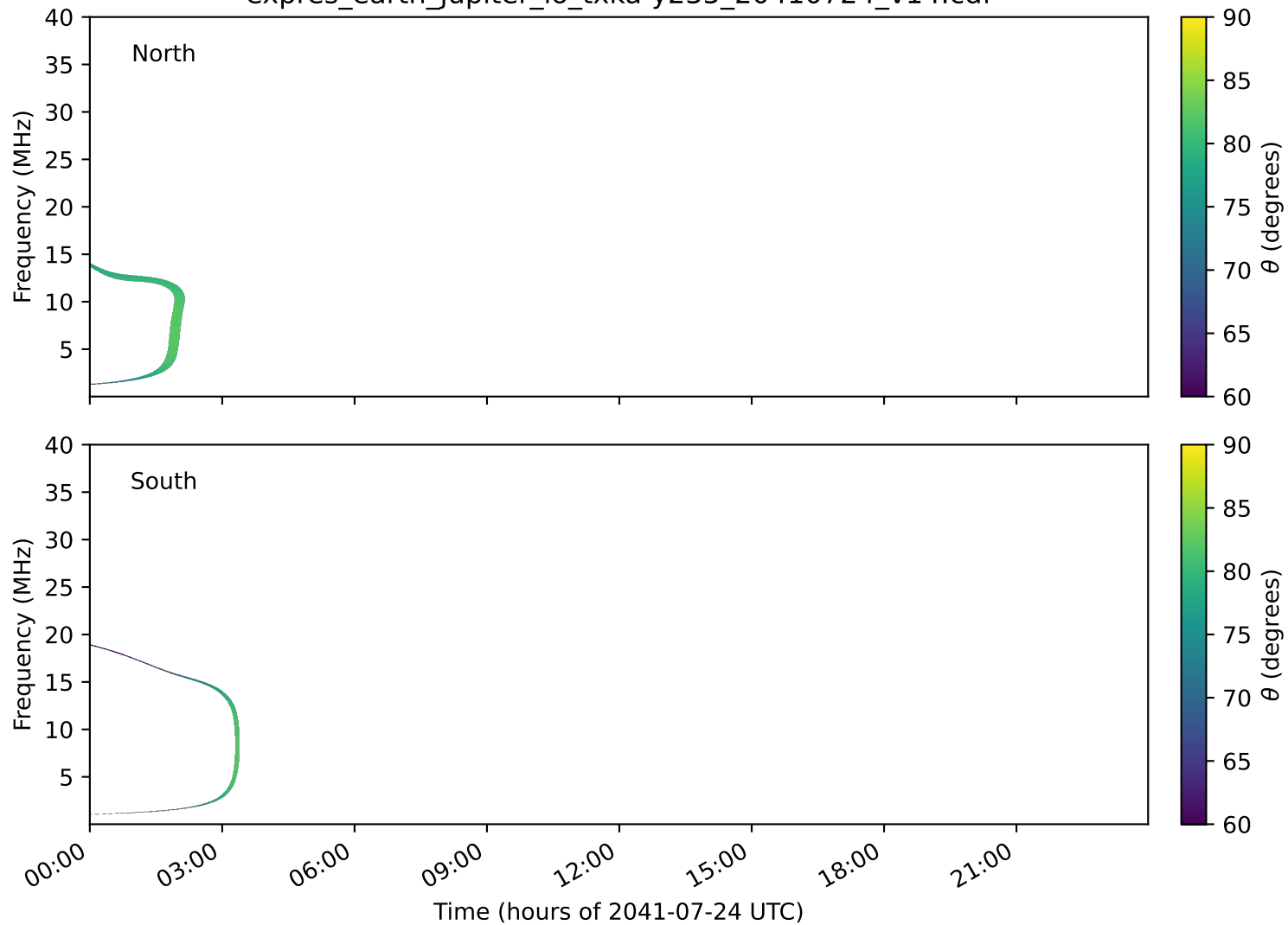
expres_earth_jupiter_io_txka-y235_20410724_v14.cdf
