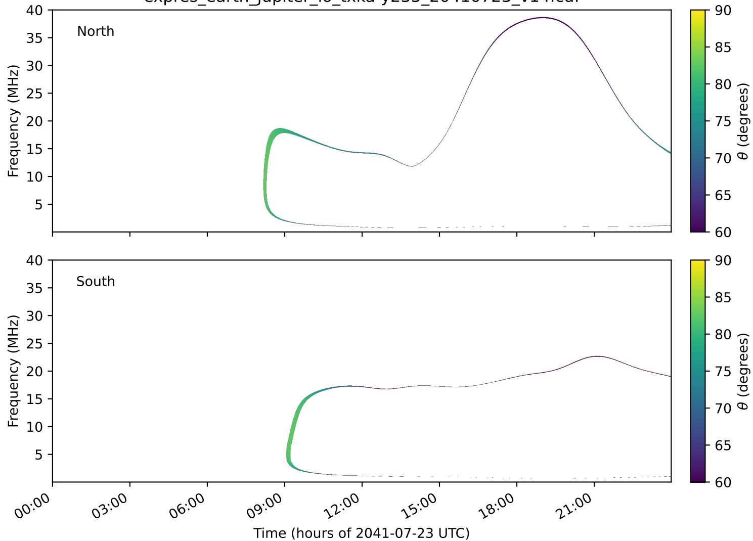
expres_earth_jupiter_io_txka-y235_20410723_v14.cdf
