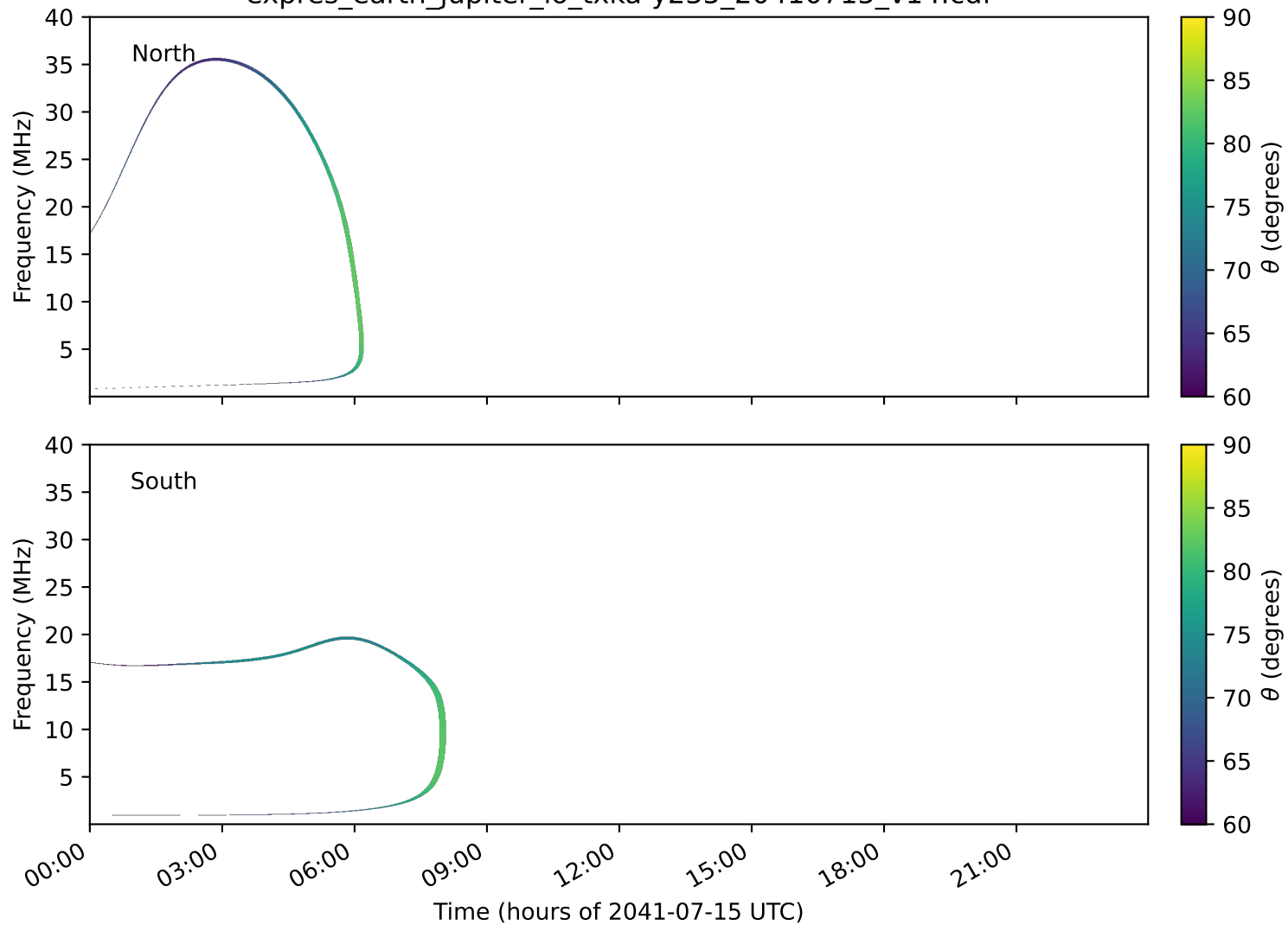
expres_earth_jupiter_io_txka-y235_20410715_v14.cdf
