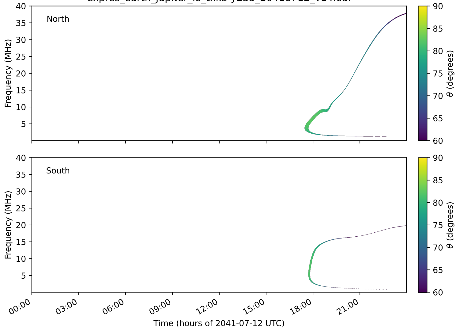
expres_earth_jupiter_io_txka-y235_20410712_v14.cdf
