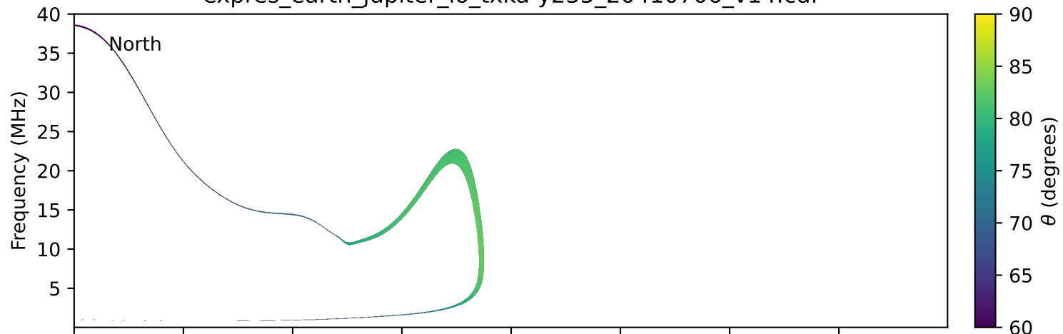
expres_earth_jupiter_io_txka-y235_20410706_v14.cdf
