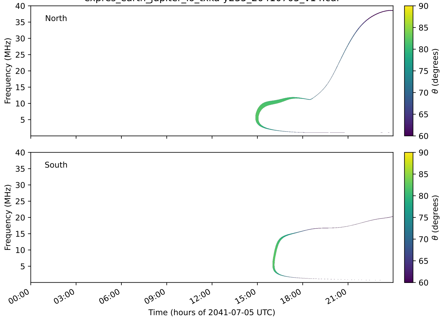
expres_earth_jupiter_io_txka-y235_20410705_v14.cdf
