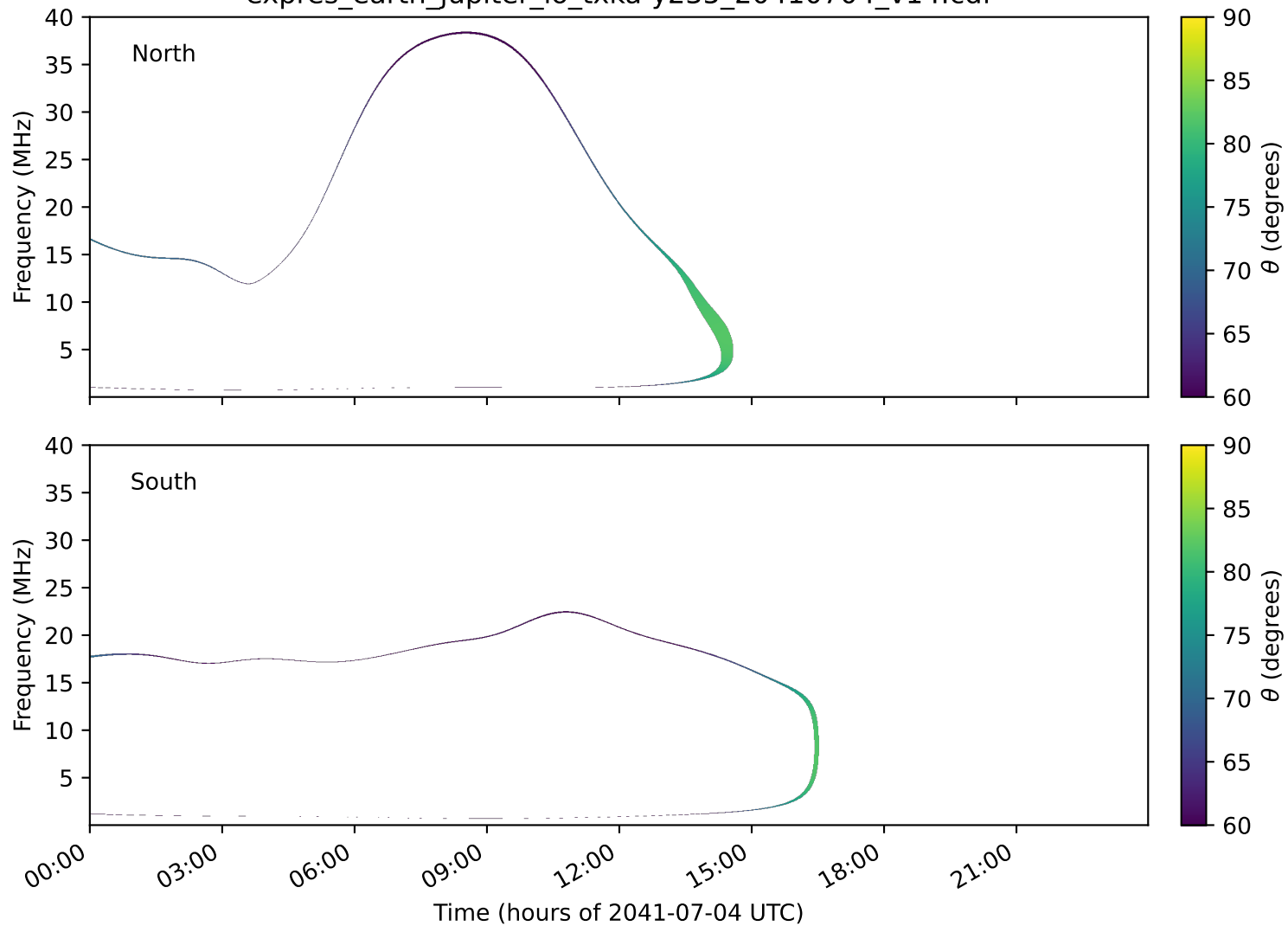
expres_earth_jupiter_io_txka-y235_20410704_v14.cdf
