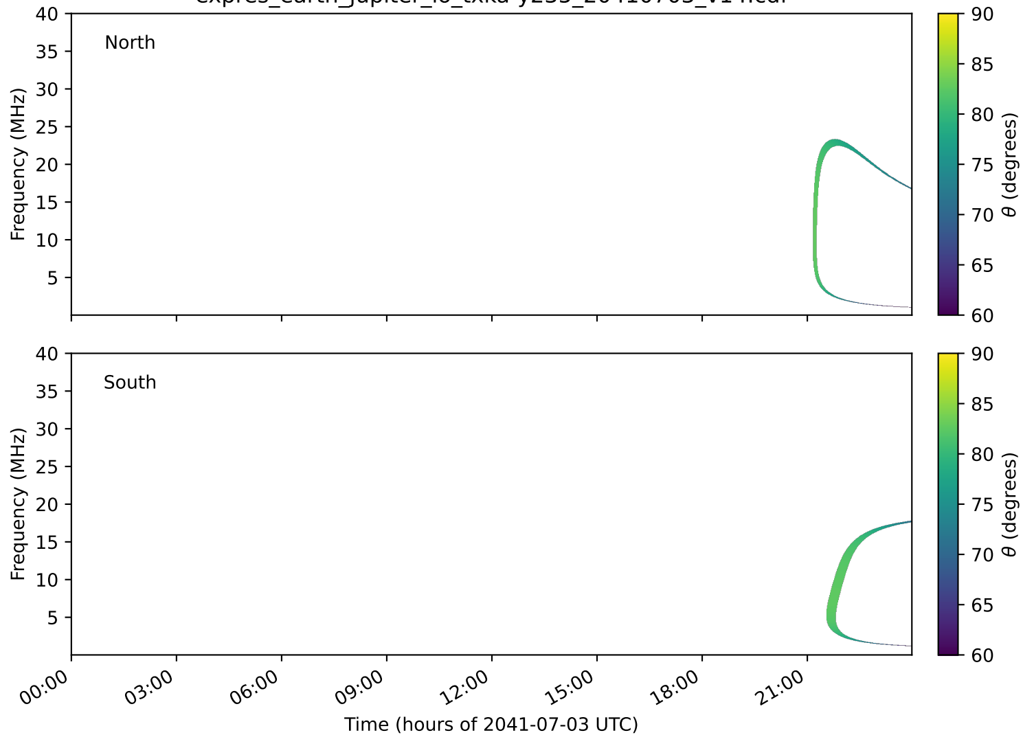
expres_earth_jupiter_io_txka-y235_20410703_v14.cdf
