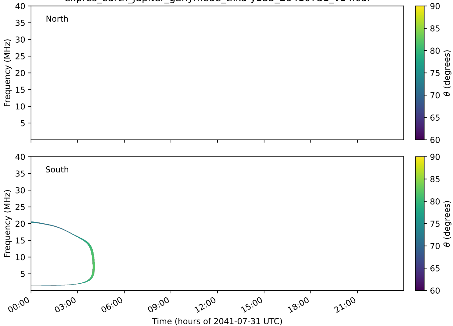
expres_earth_jupiter_ganymede_txka-y235_20410731_v14.cdf
