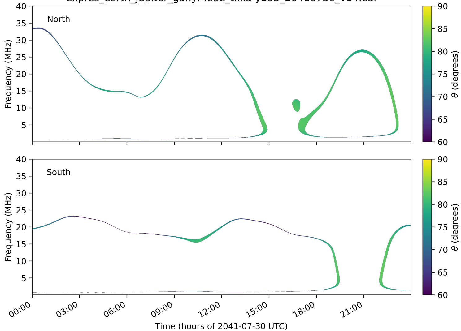
expres_earth_jupiter_ganymede_txka-y235_20410730_v14.cdf
