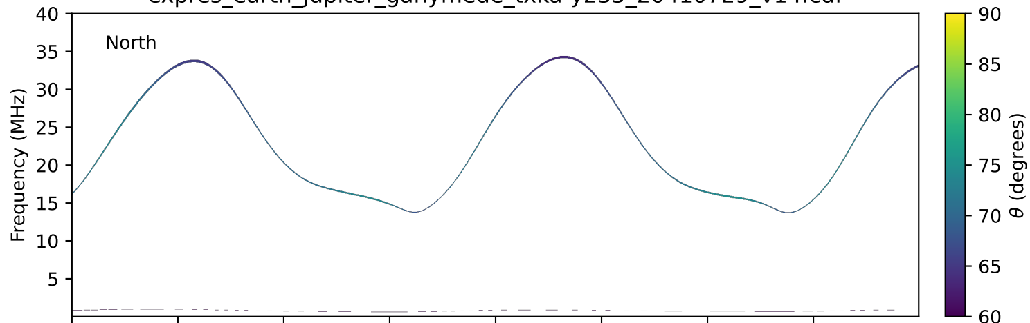
expres_earth_jupiter_ganymede_txka-y235_20410729_v14.cdf
