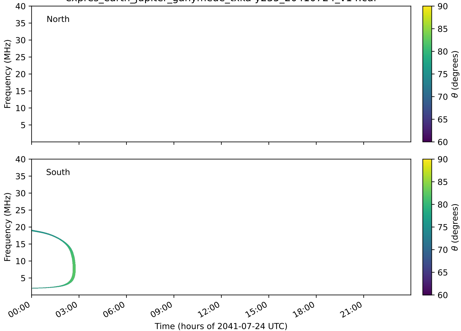
expres_earth_jupiter_ganymede_txka-y235_20410724_v14.cdf
