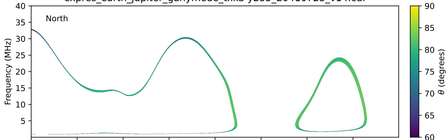
expres_earth_jupiter_ganymede_txka-y235_20410723_v14.cdf
