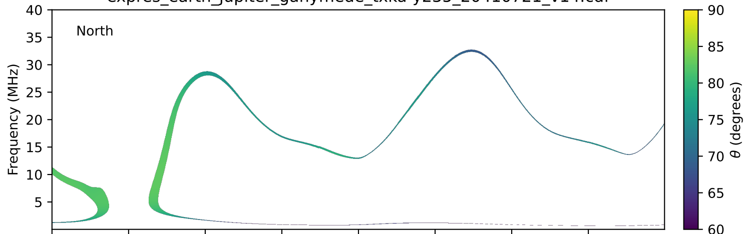
expres_earth_jupiter_ganymede_txka-y235_20410721_v14.cdf
