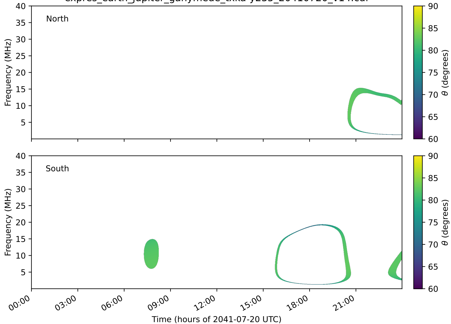
expres_earth_jupiter_ganymede_txka-y235_20410720_v14.cdf
