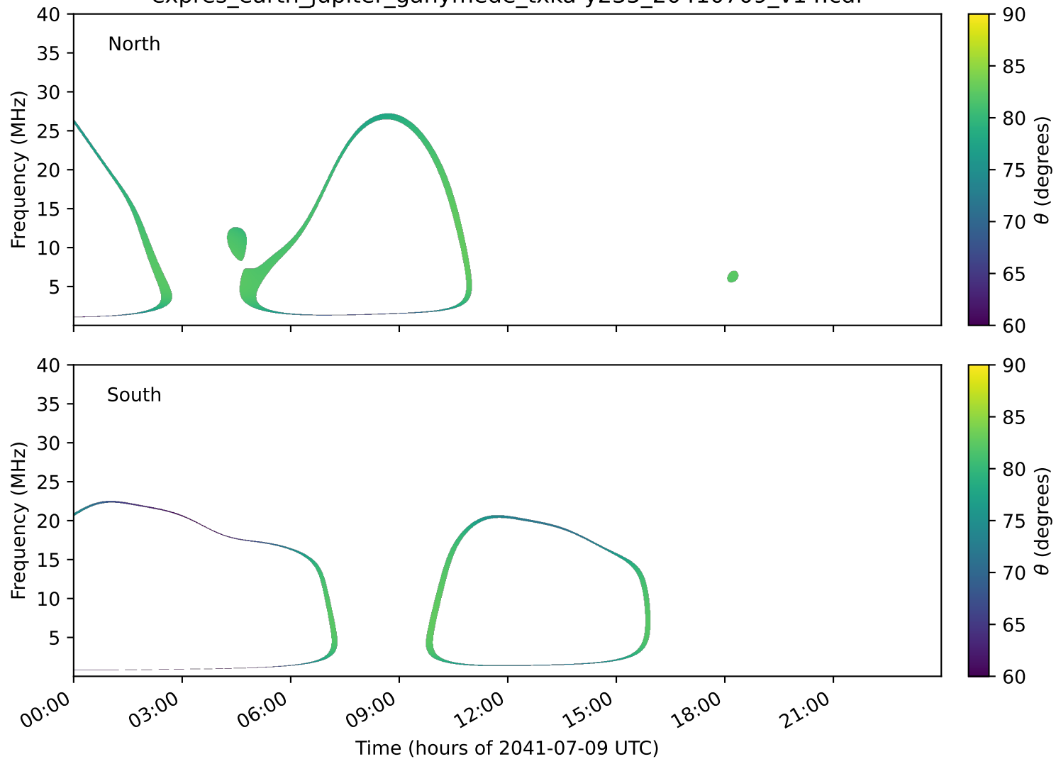
expres_earth_jupiter_ganymede_txka-y235_20410709_v14.cdf
