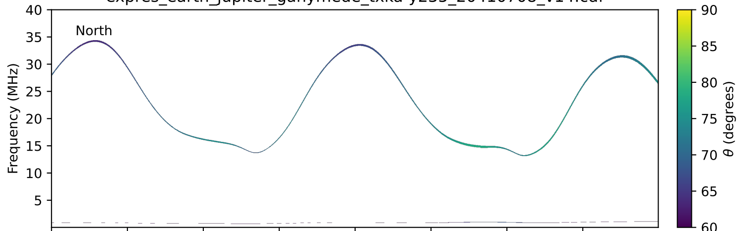
expres_earth_jupiter_ganymede_txka-y235_20410708_v14.cdf
