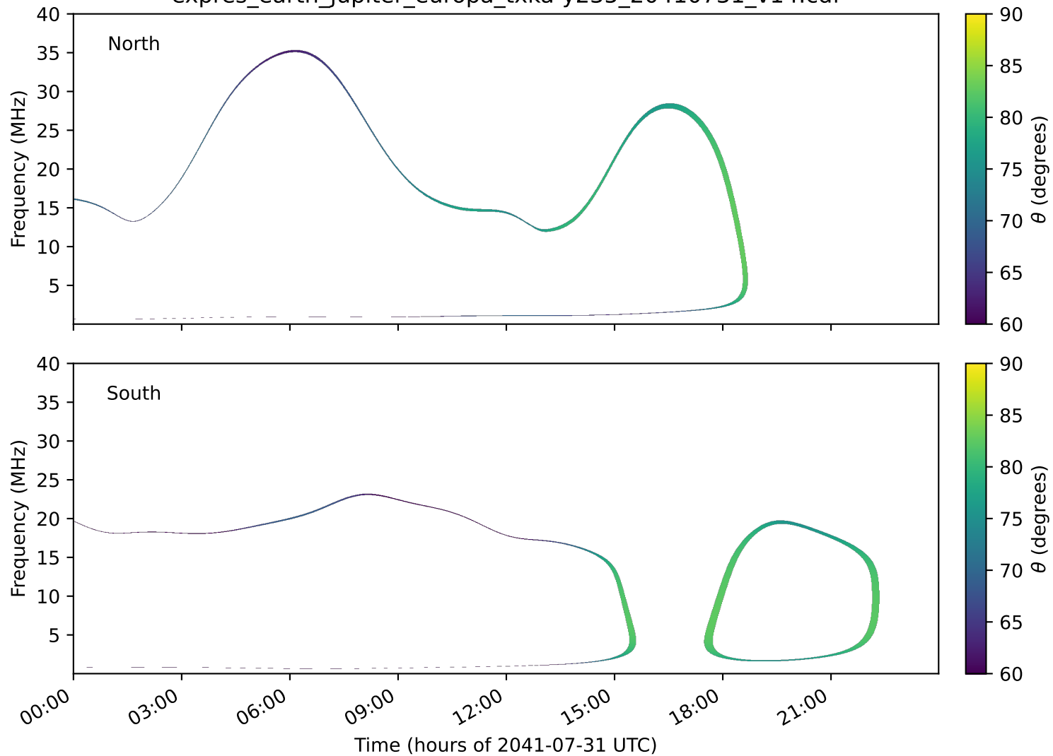
expres_earth_jupiter_europa_txka-y235_20410731_v14.cdf
