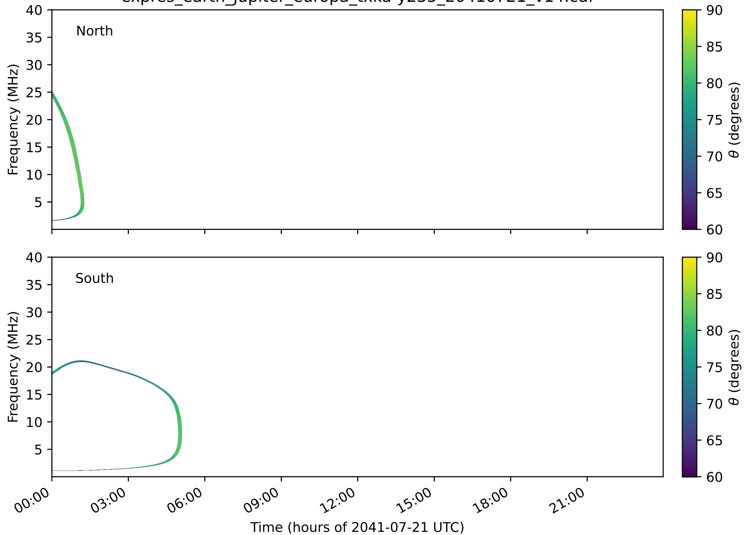
expres_earth_jupiter_europa_txka-y235_20410721_v14.cdf
