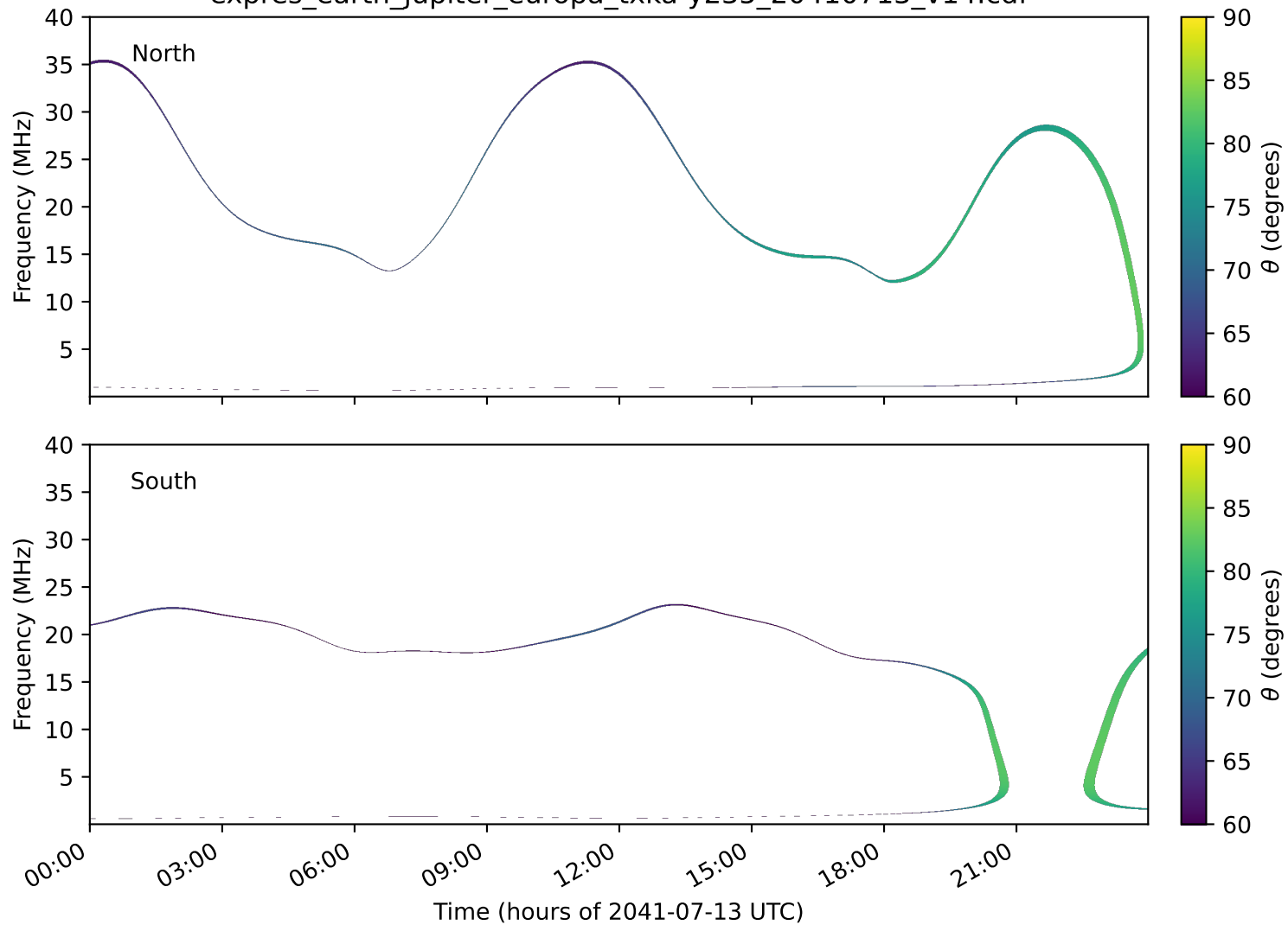
expres_earth_jupiter_europa_txka-y235_20410713_v14.cdf
