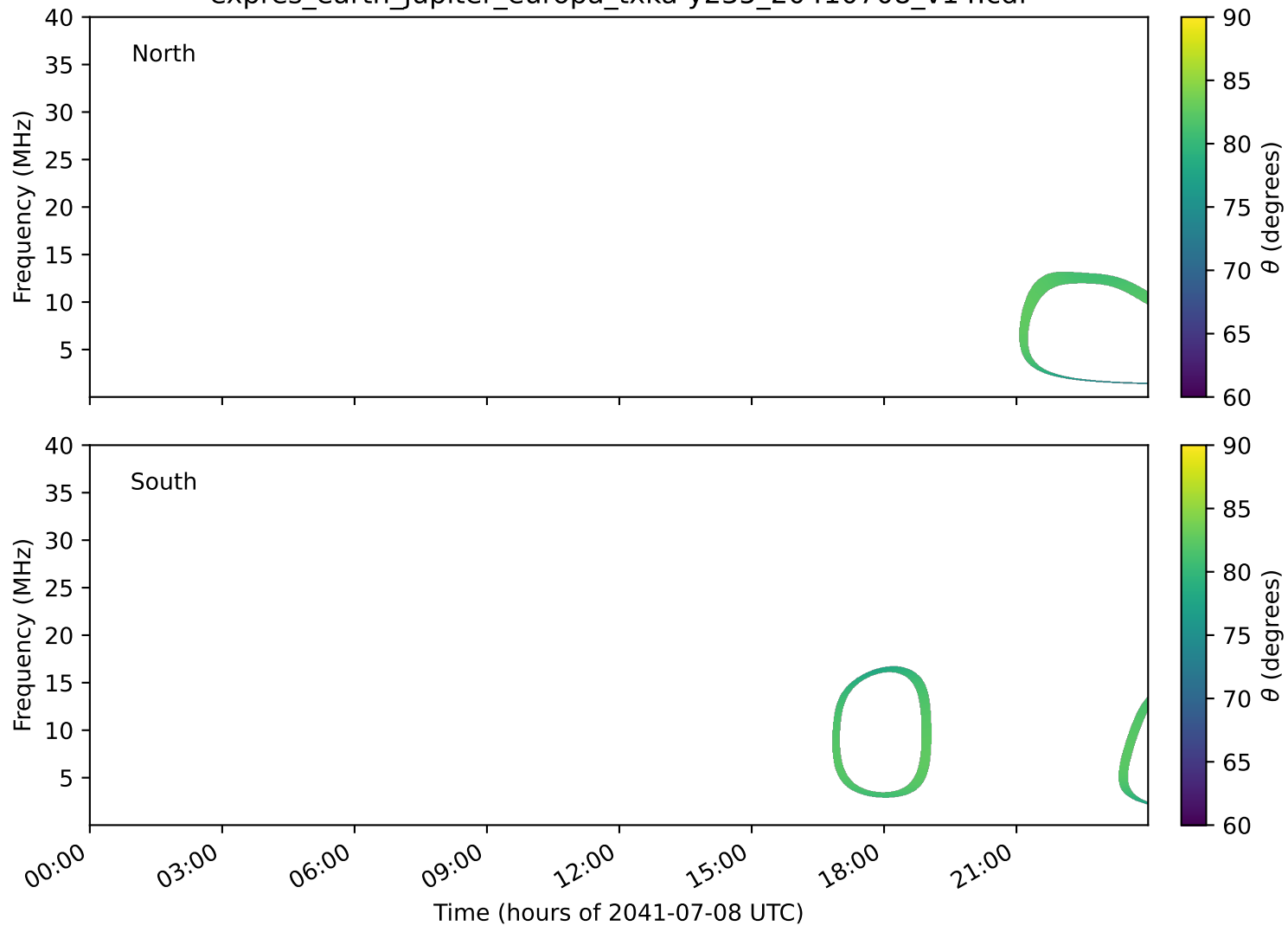
expres_earth_jupiter_europa_txka-y235_20410708_v14.cdf
