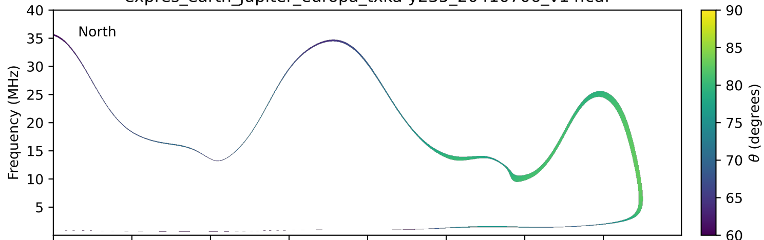
expres_earth_jupiter_europa_txka-y235_20410706_v14.cdf
