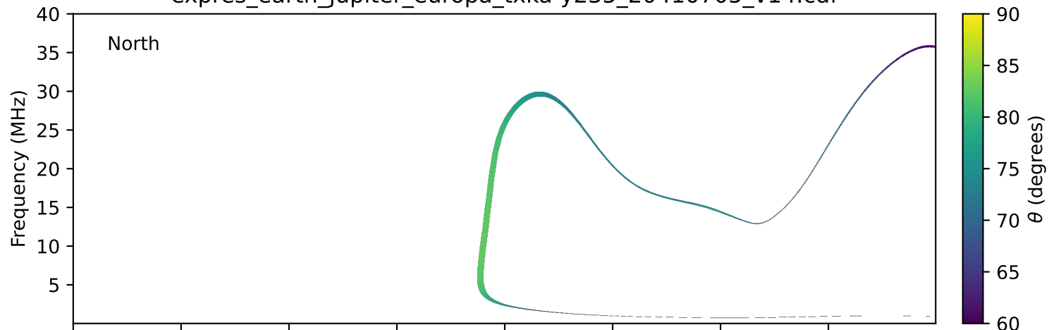
expres_earth_jupiter_europa_txka-y235_20410705_v14.cdf
