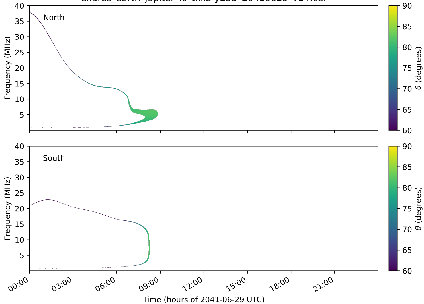
expres_earth_jupiter_io_txka-y235_20410629_v14.cdf
