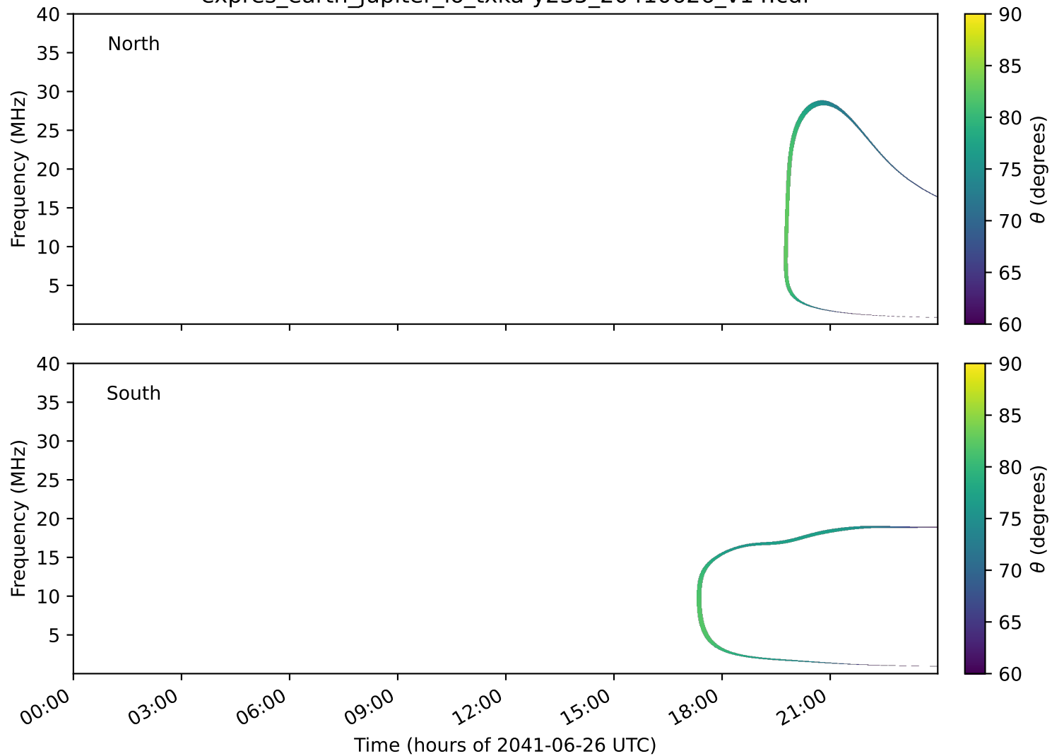
expres_earth_jupiter_io_txka-y235_20410626_v14.cdf
