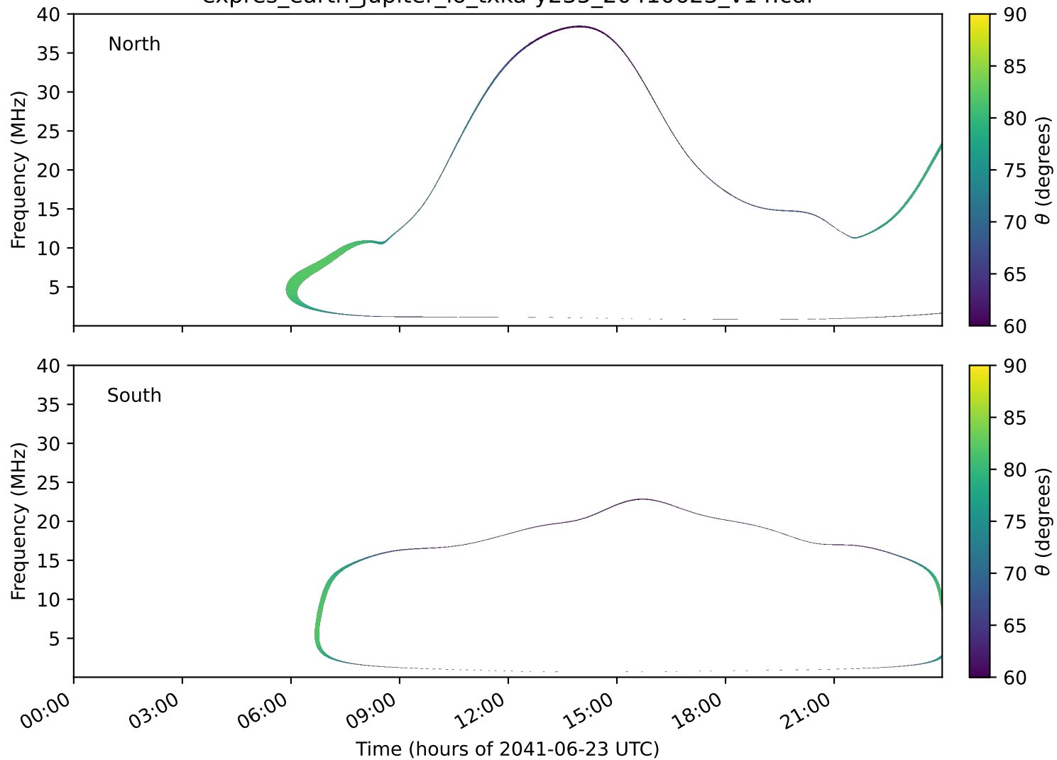
expres_earth_jupiter_io_txka-y235_20410623_v14.cdf
