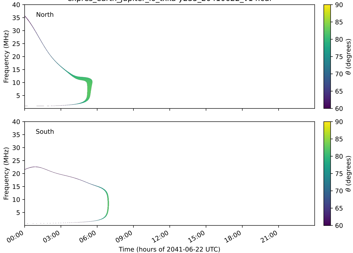
expres_earth_jupiter_io_txka-y235_20410622_v14.cdf
