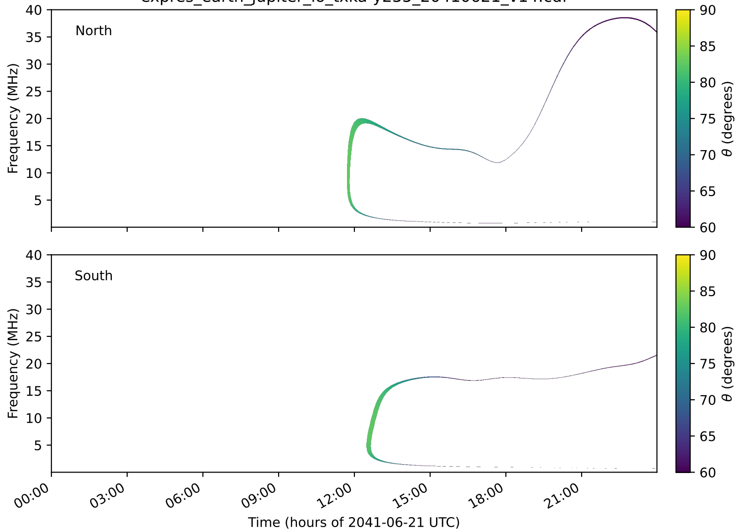
expres_earth_jupiter_io_txka-y235_20410621_v14.cdf
